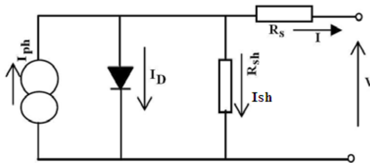
Fig.1. Electrical model of a PV generator with five parameters [1,4]
