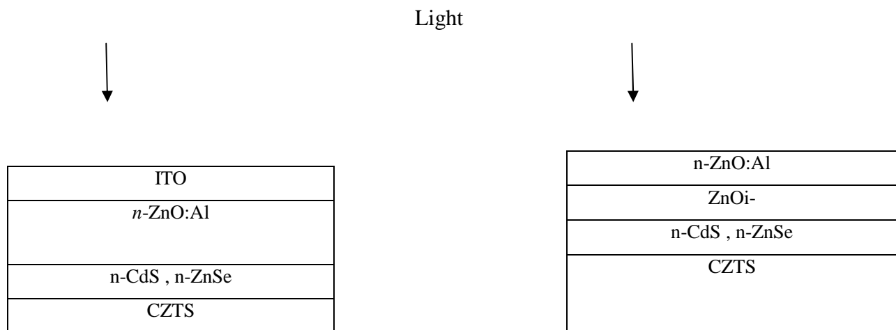
Fig.2. Structure of Solar cell
