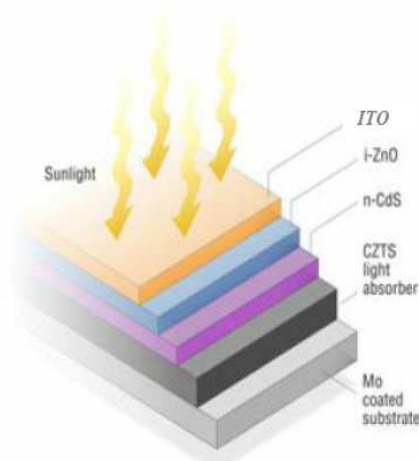
Fig.1. Structure of a photovoltaic cell CZTS
