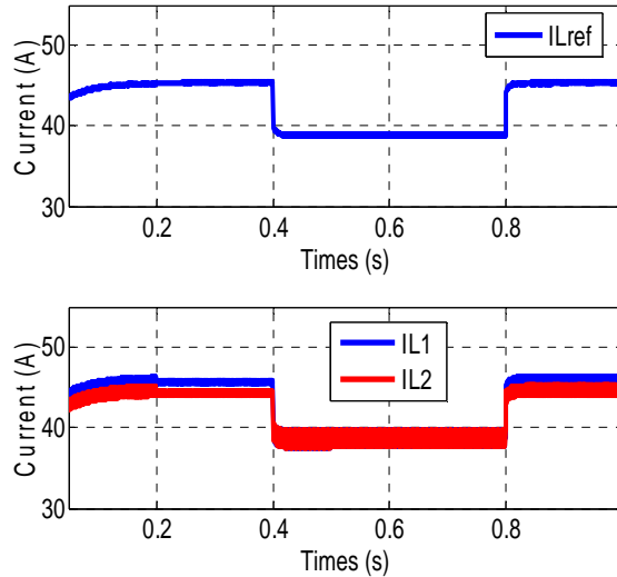
Fig.11. Inductor currents while the load change
