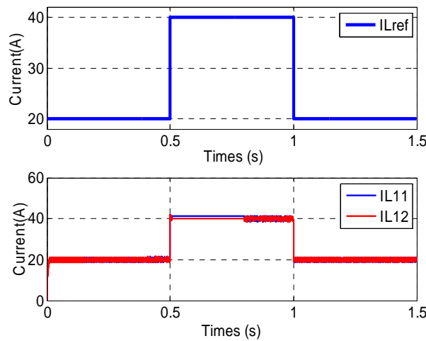
Fig.6. Sliding-mode controller dynamic response while the variation of inductor current from 20 to 40 A
